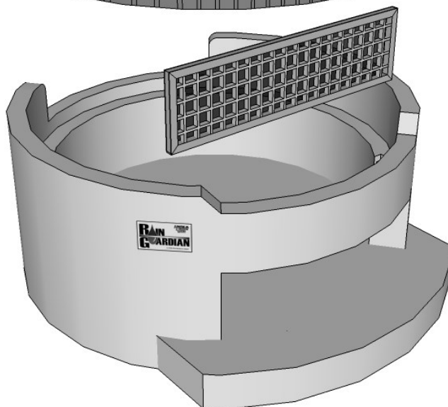
Steel reinforced monolithic concrete riser and base (1,030 lbs.)
