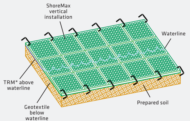
FIGURE 8: Edge of mat anchoring
