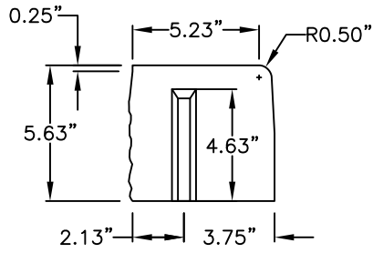
SIDE VIEW "A"
