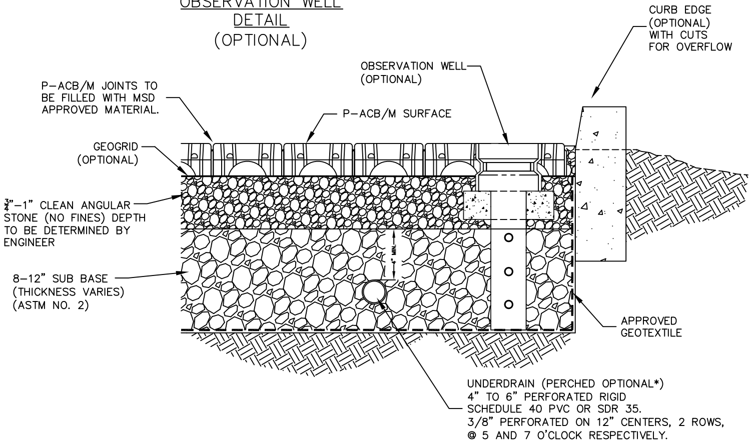
PERMEABLE - ARTICULATING CONCRETE BLOCK/MAT TYPICAL SECTION
