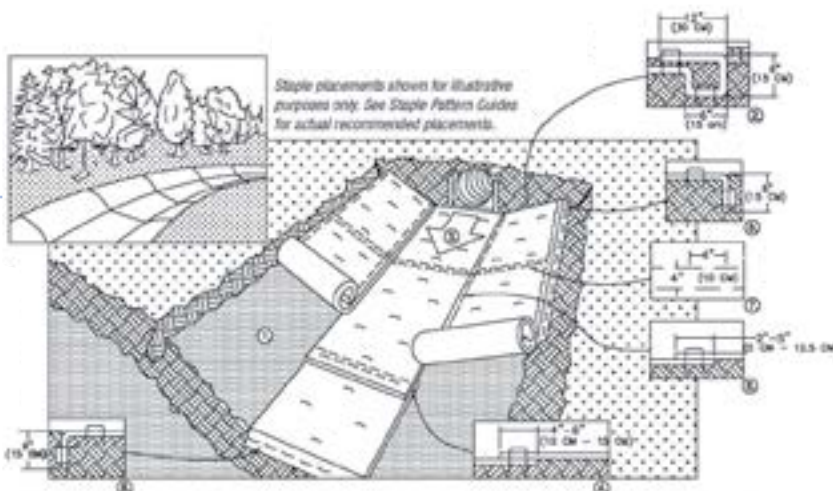
Standard installation details.
