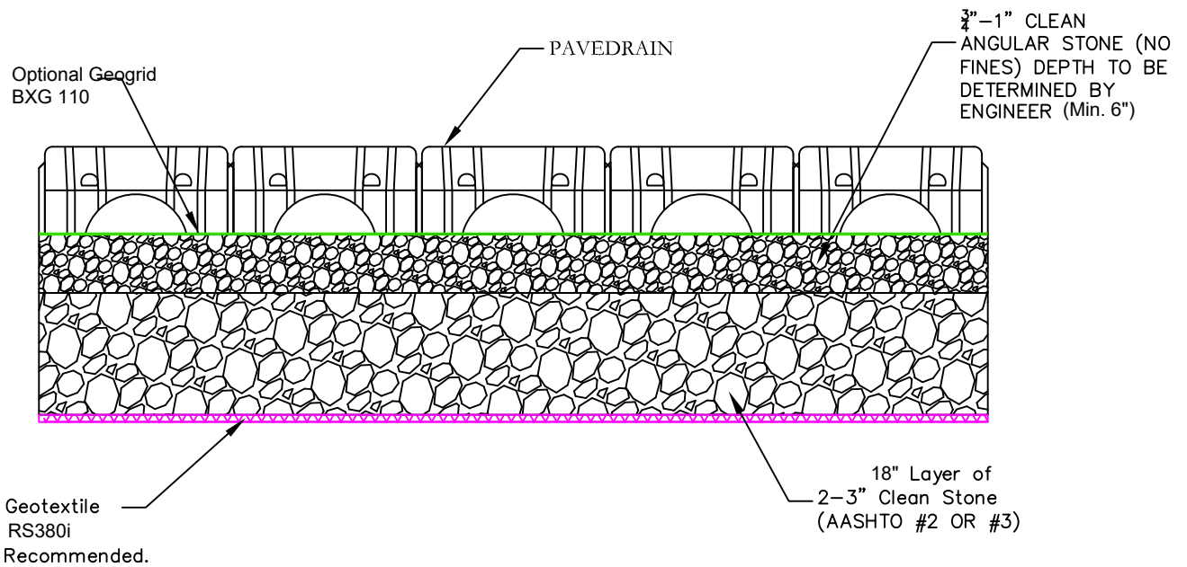
CROSS-SECTION END VIEW
