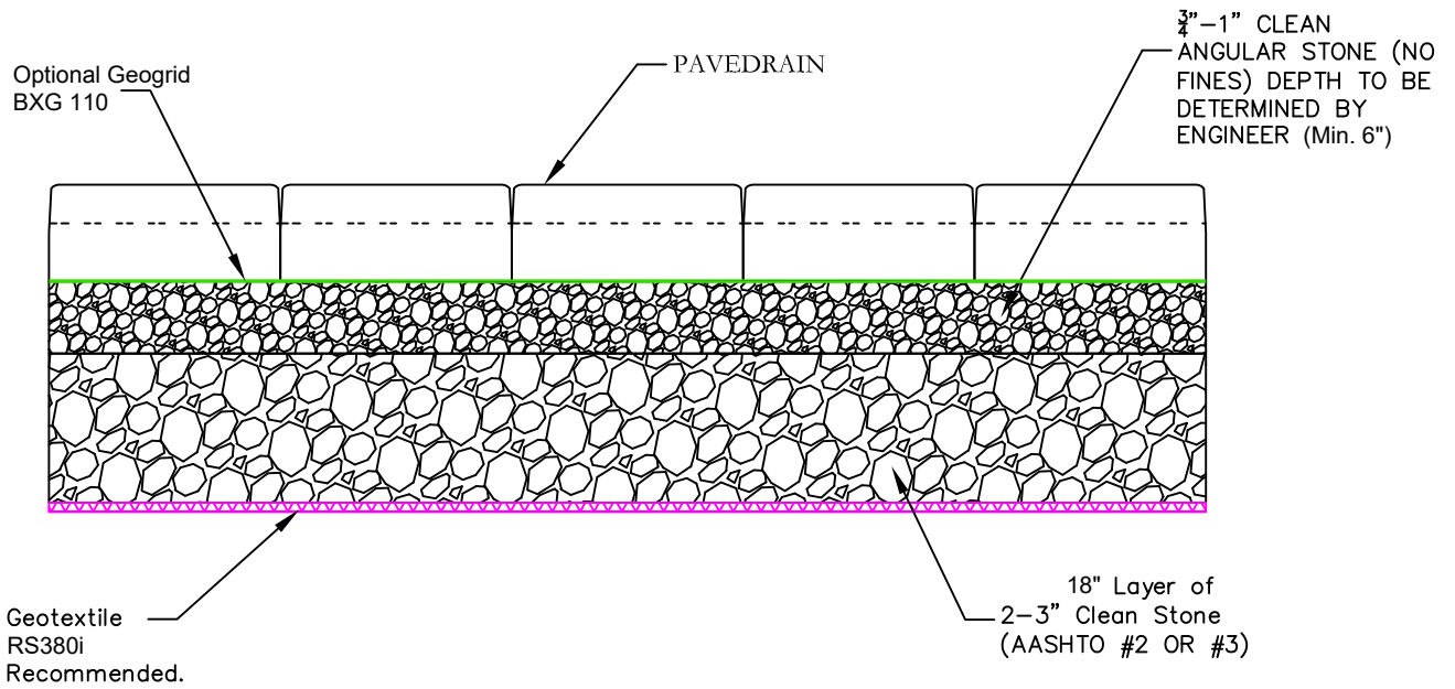
CROSS-SECTION SIDE VIEW
