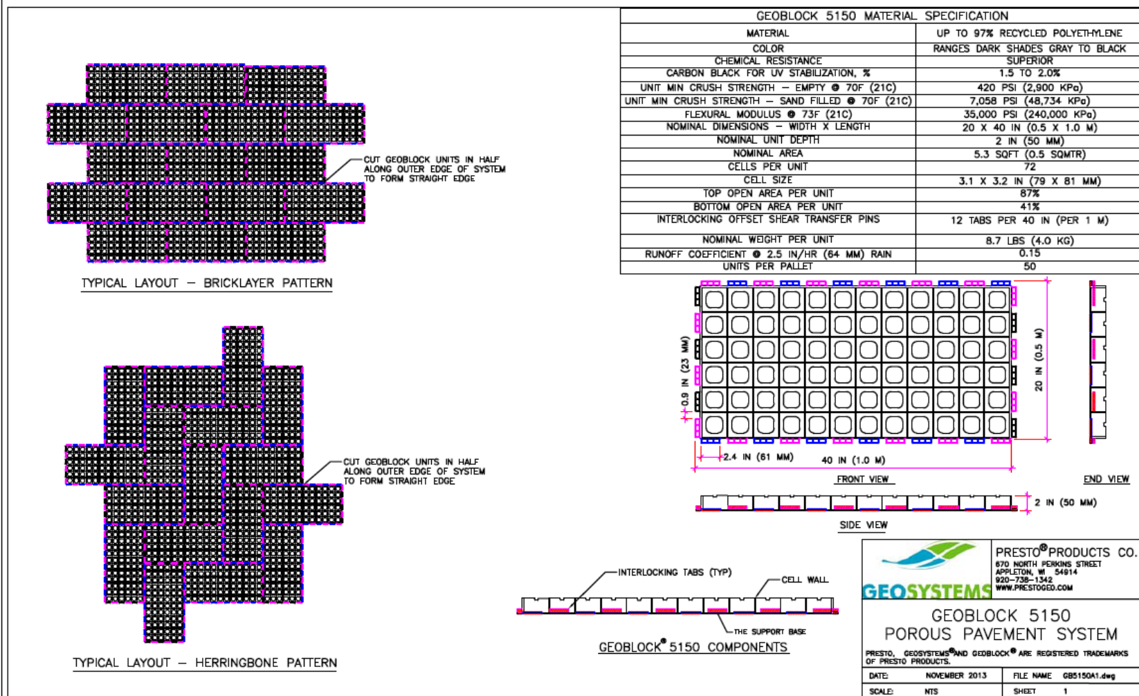
Figure 4 Geoblock ® 5150 System Material Specification and Layout
