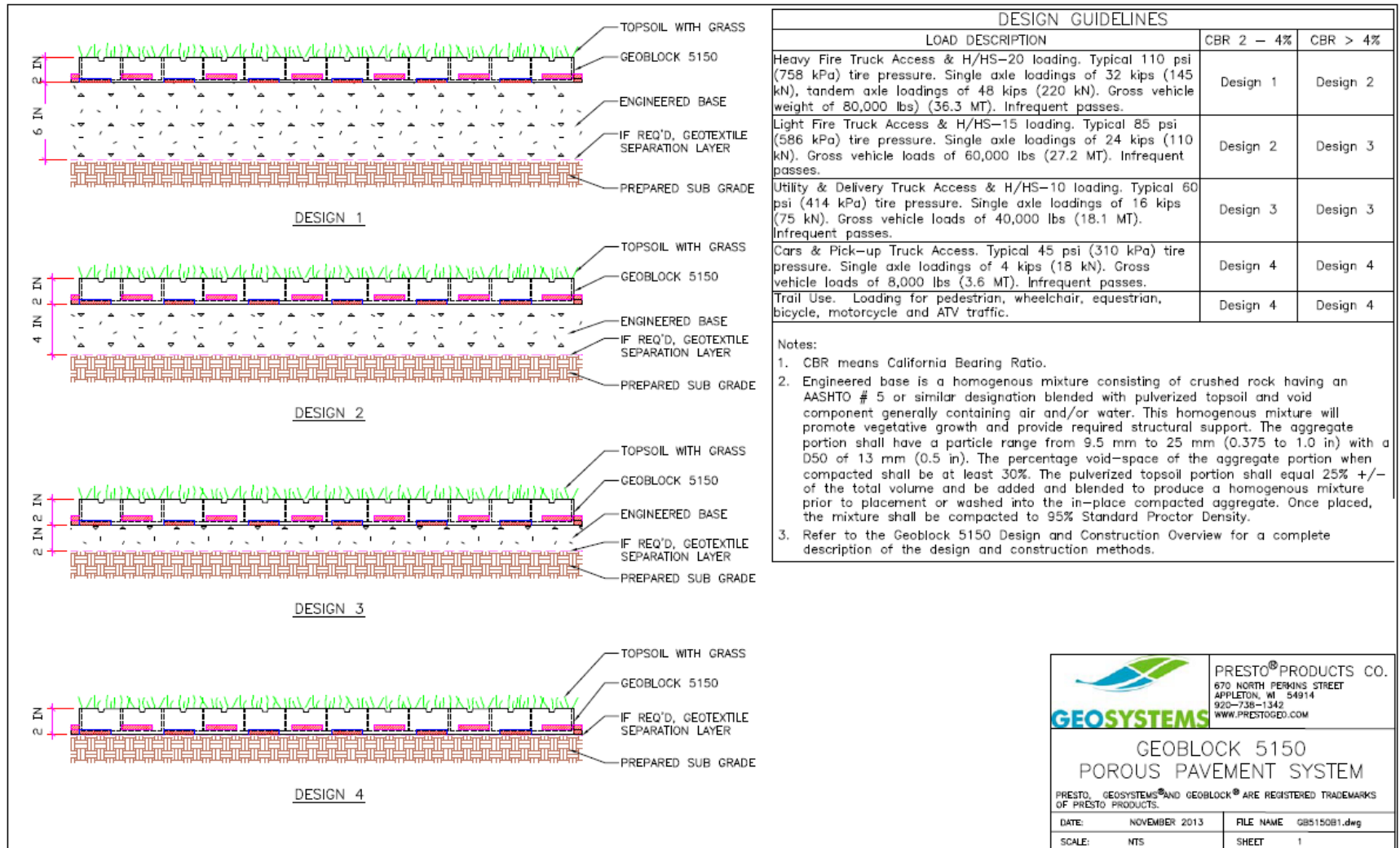
Figure 5 Geoblock®5150 System Usage Guideline
